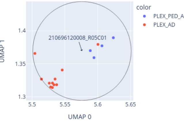
Close-up of UMAP for 210696120008_R05C01 reference: AllIDATv2_20210804_HPAP_Sarc.xlsx (19967 cases), 0 CpGs
