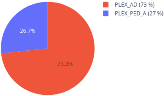
Neighbors in UMAP for 210696120008_R05C01 reference: AllIDATv2_20210804_HPAP_Sarc.xlsx (19967 cases), 0 CpGs
