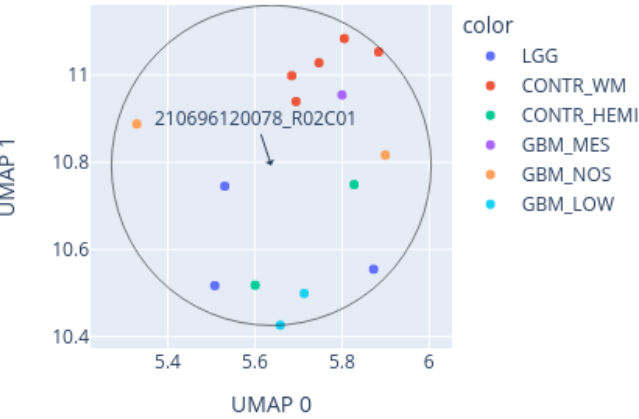
Close-up of UMAP for 210696120078_R02C01 reference: AllIDATv2_20210804_HPAP_Sarc.xlsx (19967 cases), 0 CpGs
