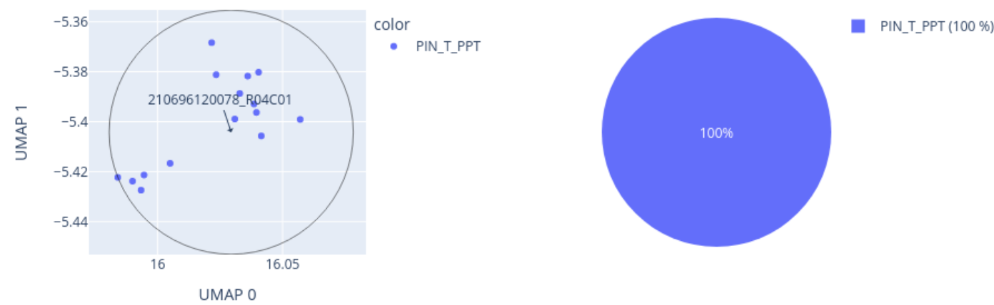
Close-up of UMAP for 210696120078_R04C01 reference: AllIDATv2_20210804_HPAP_Sarc.xlsx (19967 cases), 0 CpGs
