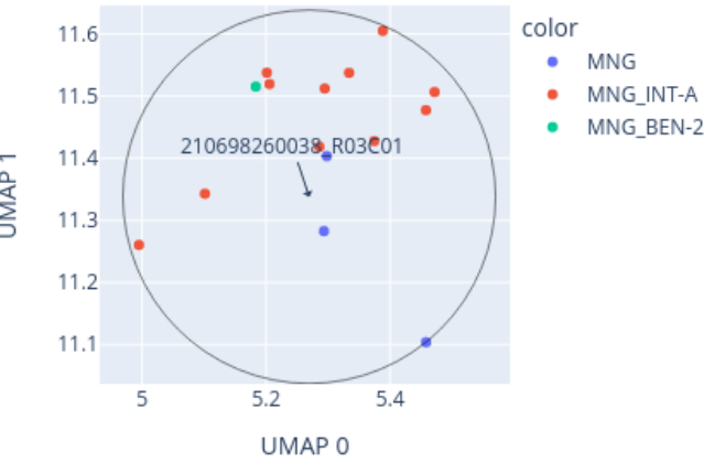
Close-up of UMAP for 210698260038_R03C01 reference: AllIDATv2_20210804_HPAP_Sarc.xlsx (19967 cases), 0 CpGs
