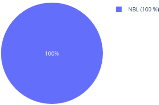
Neighbors in UMAP for 210698260039_R07C01 reference: AllIDATv2_20210804_HPAP_Sarc.xlsx (19967 cases), 0 CpGs
