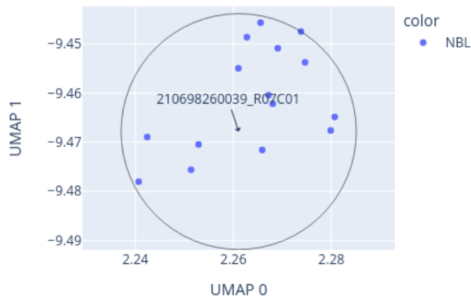
Close-up of UMAP for 210698260039_R07C01 reference: AllIDATv2_20210804_HPAP_Sarc.xlsx (19967 cases), 0 CpGs
