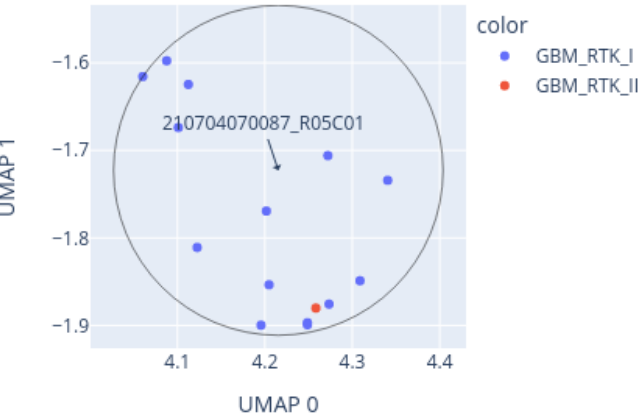
Close-up of UMAP for 210704070087_R05C01 reference: GSE90496_lfp02.xlsx (2980 cases), 0 CpGs
