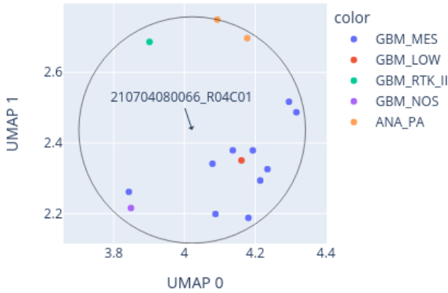
Close-up of UMAP for 210704080066_R04C01 reference: AllIDATv2_20210804_HPAP_Sarc.xlsx (19967 cases), 0 CpGs
