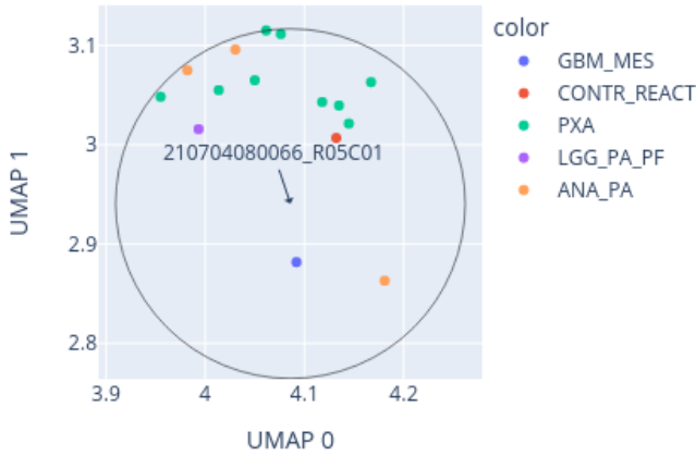
Close-up of UMAP for 210704080066_R05C01 reference: AllIDATv2_20210804_HPAP_Sarc.xlsx (19967 cases), 0 CpGs
