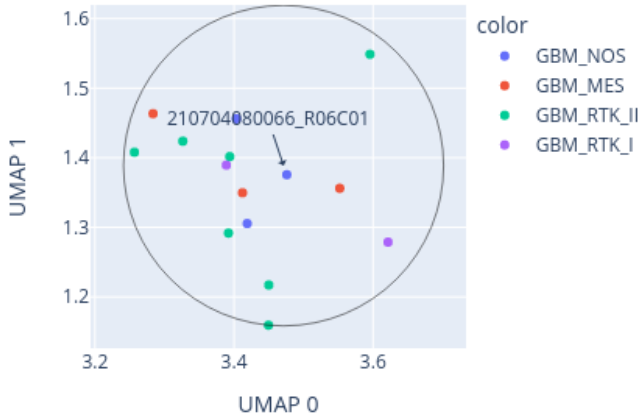
Close-up of UMAP for 210704080066_R06C01 reference: AllIDATv2_20210804_HPAP_Sarc.xlsx (19967 cases), 0 CpGs
