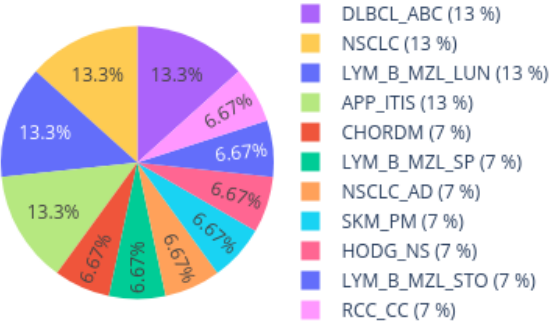
Neighbors in UMAP for 210711060002_R08C01 reference: AllIDATv2_20210804_HPAP_Sarc.xlsx (19967 cases), 0 CpGs
