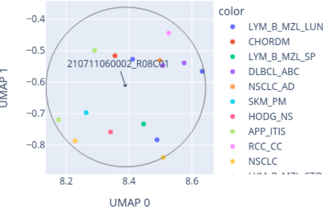
Close-up of UMAP for 210711060002_R08C01 reference: AllIDATv2_20210804_HPAP_Sarc.xlsx (19967 cases), 0 CpGs
