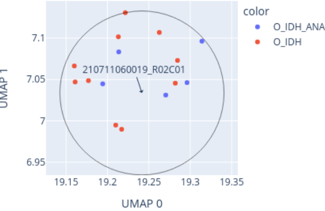
Close-up of UMAP for 210711060019_R02C01 reference: AllIDATv2_20210804_HPAP_Sarc.xlsx (19967 cases), 0 CpGs
