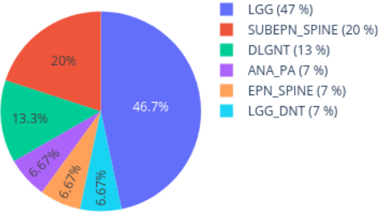
Neighbors in UMAP for 210711060044_R01C01 reference: AllIDATv2_20210804_HPAP_Sarc.xlsx (19967 cases), 0 CpGs
