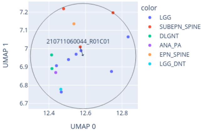
Close-up of UMAP for 210711060044_R01C01 reference: AllIDATv2_20210804_HPAP_Sarc.xlsx (19967 cases), 0 CpGs
