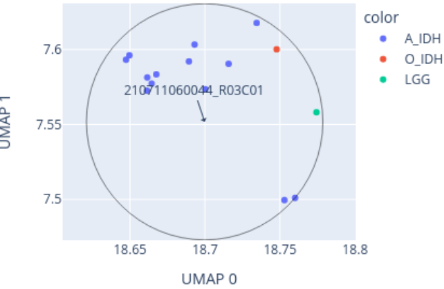
Close-up of UMAP for 210711060044_R03C01 reference: AllIDATv2_20210804_HPAP_Sarc.xlsx (19967 cases), 0 CpGs
