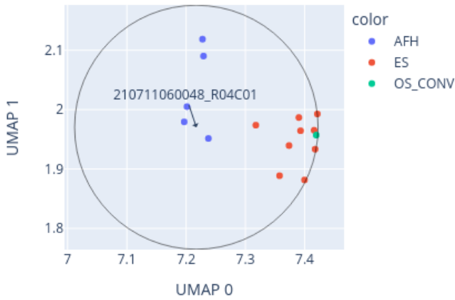
Close-up of UMAP for 210711060048_R04C01 reference: AllIDATv2_20210804_HPAP_Sarc.xlsx (19967 cases), 0 CpGs
