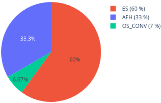
Neighbors in UMAP for 210711060048_R04C01 reference: AllIDATv2_20210804_HPAP_Sarc.xlsx (19967 cases), 0 CpGs
