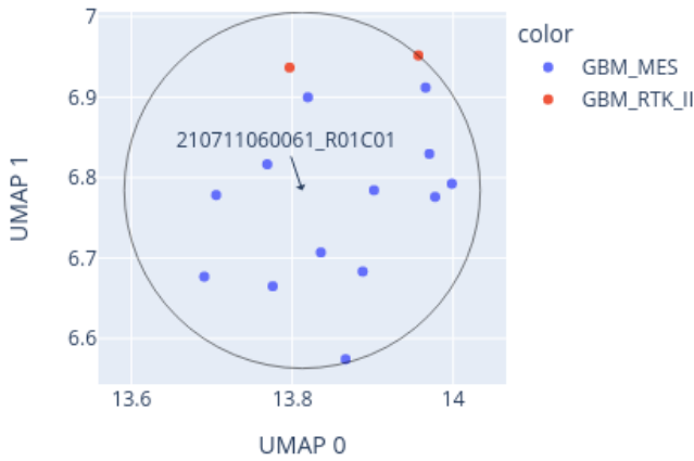
Close-up of UMAP for 210711060061_R01C01 reference: AllIDATv2_20210804_HPAP_Sarc.xlsx (19967 cases), 0 CpGs
