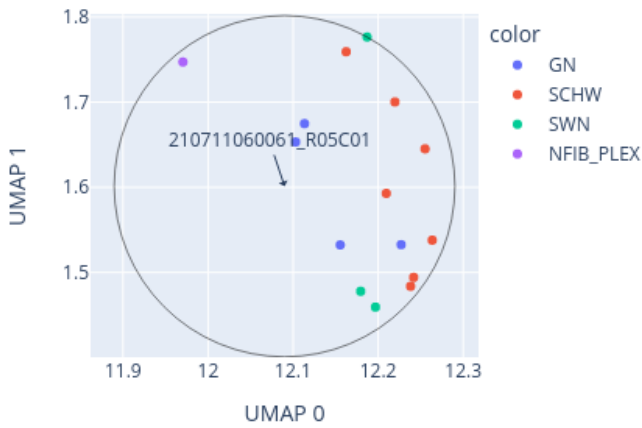
Close-up of UMAP for 210711060061_R05C01 reference: AllIDATv2_20210804_HPAP_Sarc.xlsx (19967 cases), 0 CpGs
