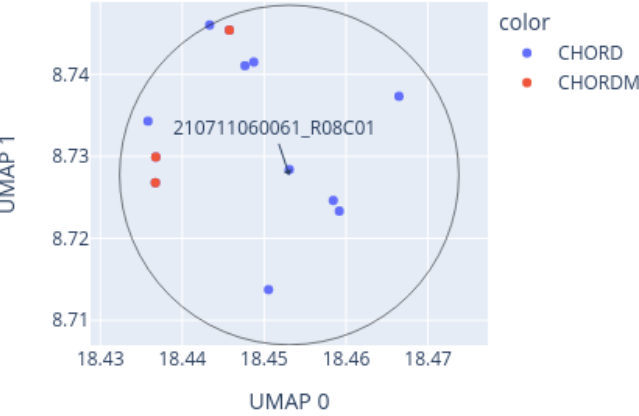
Close-up of UMAP for 210711060061_R08C01 reference: AllIDATv2_20210804_HPAP_Sarc.xlsx (19967 cases), 0 CpGs
