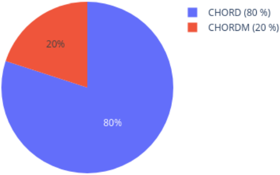
Neighbors in UMAP for 210711060061_R08C01 reference: AllIDATv2_20210804_HPAP_Sarc.xlsx (19967 cases), 0 CpGs
