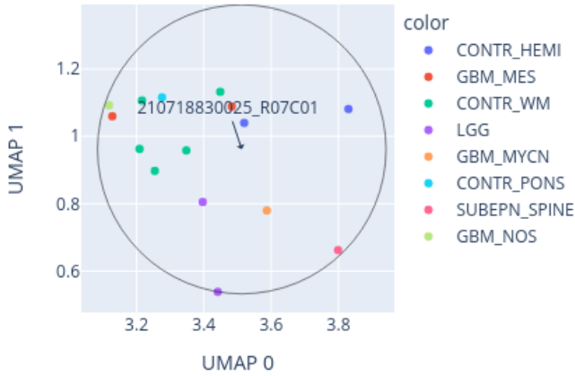
Close-up of UMAP for 210718830025_R07C01 reference: AllIDATv2_20210804_HPAP_Sarc.xlsx (19967 cases), 0 CpGs
