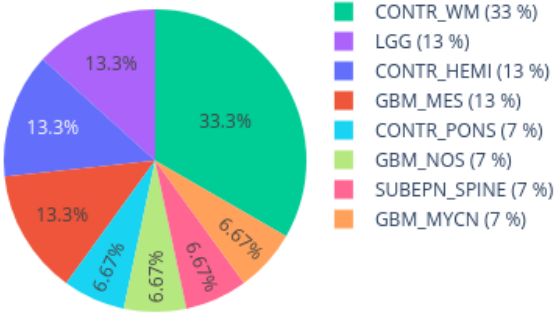
Neighbors in UMAP for 210718830025_R07C01 reference: AllIDATv2_20210804_HPAP_Sarc.xlsx (19967 cases), 0 CpGs
