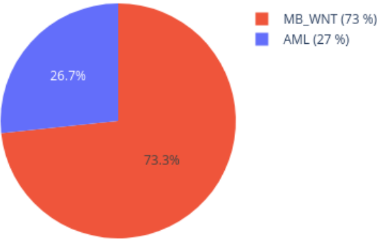
Neighbors in UMAP for 210718830077_R04C01 reference: AllIDATv2_20210804_HPAP_Sarc.xlsx (19967 cases), 0 CpGs
