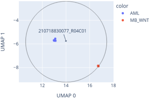
Close-up of UMAP for 210718830077_R04C01 reference: AllIDATv2_20210804_HPAP_Sarc.xlsx (19967 cases), 0 CpGs
