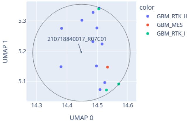
Close-up of UMAP for 210718840017_R07C01 reference: AllIDATv2_20210804_HPAP_Sarc.xlsx (19967 cases), 0 CpGs
