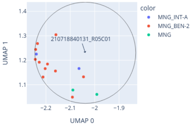
Close-up of UMAP for 210718840131_R05C01 reference: AllIDATv2_20210804_HPAP_Sarc.xlsx (19967 cases), 0 CpGs
