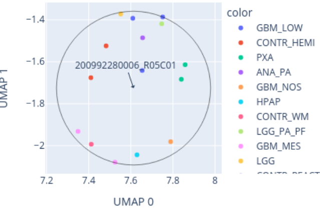
Close-up of UMAP for 200992280006_R05C01 reference: AllIDATv2_20210804_HPAP_Sarc.xlsx (19967 cases), 0 CpGs
