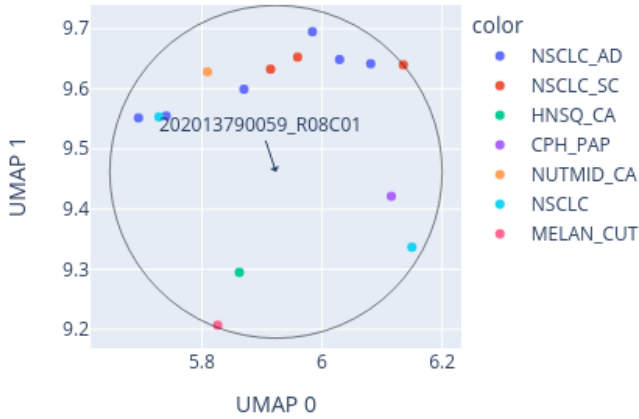
Close-up of UMAP for 202013790059_R08C01 reference: AllIDATv2_20210804_HPAP_Sarc.xlsx (19967 cases), 0 CpGs
