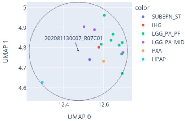
Close-up of UMAP for 202081130007_R07C01 reference: AllIDATv2_20210804_HPAP_Sarc.xlsx (19967 cases), 0 CpGs
