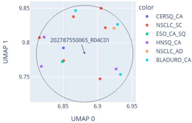
Close-up of UMAP for 202787550065_R04C01 reference: AllIDATv2_20210804_HPAP_Sarc.xlsx (19967 cases), 0 CpGs
