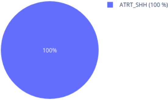
Neighbors in UMAP for 203020780081_R05C01 reference: AllIDATv2_20210804_HPAP_Sarc.xlsx (19967 cases), 0 CpGs
