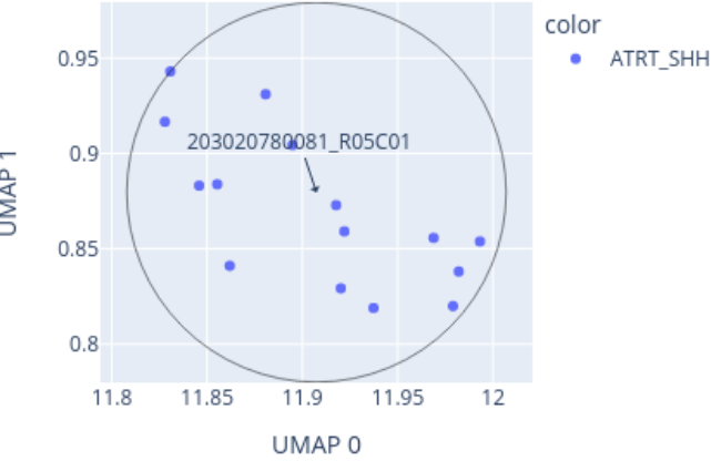
Close-up of UMAP for 203020780081_R05C01 reference: AllIDATv2_20210804_HPAP_Sarc.xlsx (19967 cases), 0 CpGs
