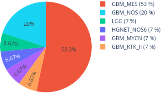
Neighbors in UMAP for 203020900031_R01C01 reference: AllIDATv2_20210804_HPAP_Sarc.xlsx (19967 cases), 0 CpGs
