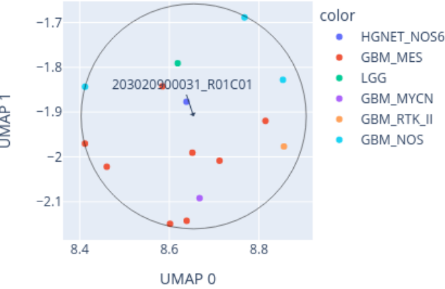
Close-up of UMAP for 203020900031_R01C01 reference: AllIDATv2_20210804_HPAP_Sarc.xlsx (19967 cases), 0 CpGs
