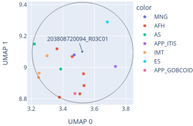
Close-up of UMAP for 203808720094_R03C01 reference: AllIDATv2_20210804_HPAP_Sarc.xlsx (19967 cases), 0 CpGs
