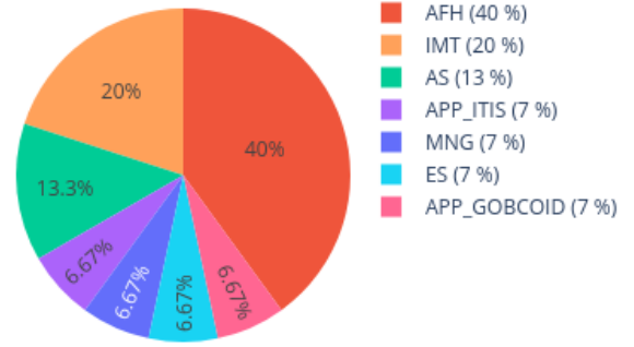
Neighbors in UMAP for 203808720094_R03C01 reference: AllIDATv2_20210804_HPAP_Sarc.xlsx (19967 cases), 0 CpGs
