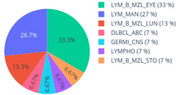
Neighbors in UMAP for 203808720094_R06C01 reference: AllIDATv2_20210804_HPAP_Sarc.xlsx (19967 cases), 0 CpGs
