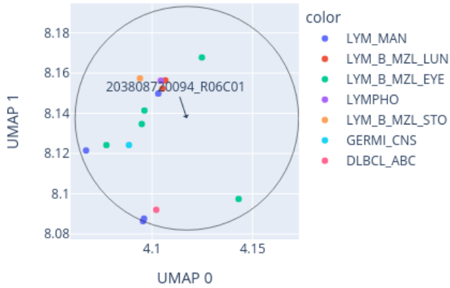
Close-up of UMAP for 203808720094_R06C01 reference: AllIDATv2_20210804_HPAP_Sarc.xlsx (19967 cases), 0 CpGs
