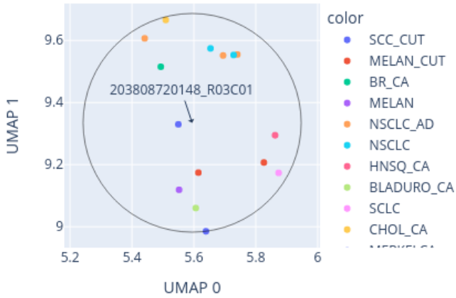
Close-up of UMAP for 203808720148_R03C01 reference: AllIDATv2_20210804_HPAP_Sarc.xlsx (19967 cases), 0 CpGs
