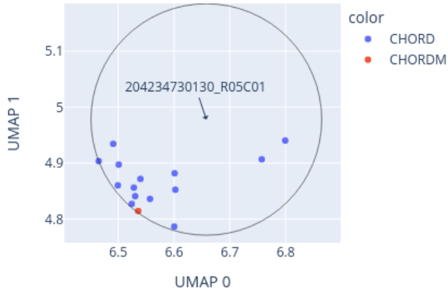
Close-up of UMAP for 204234730130_R05C01 reference: AllIDATv2_20210804_HPAP_Sarc.xlsx (19967 cases), 0 CpGs
