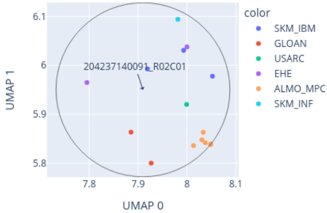
Close-up of UMAP for 204237140091_R02C01 reference: AllIDATv2_20210804_HPAP_Sarc.xlsx (19967 cases), 0 CpGs
