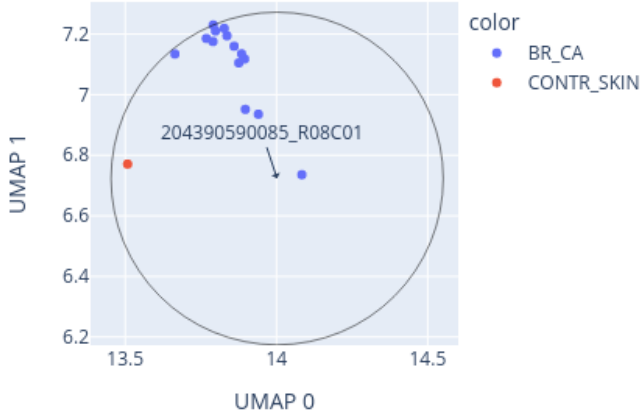
Close-up of UMAP for 204390590085_R08C01 reference: AllIDATv2_20210804_HPAP_Sarc.xlsx (19967 cases), 0 CpGs
