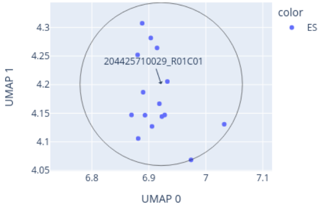
Close-up of UMAP for 204425710029_R01C01 reference: AllIDATv2_20210804_HPAP_Sarc.xlsx (19967 cases), 0 CpGs
