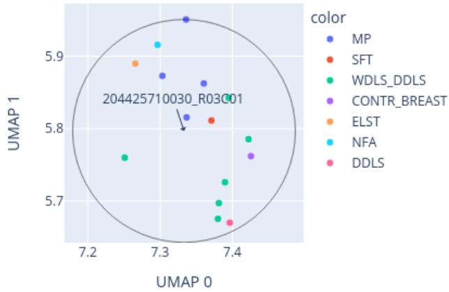
Close-up of UMAP for 204425710030_R03C01 reference: AllIDATv2_20210804_HPAP_Sarc.xlsx (19967 cases), 0 CpGs
