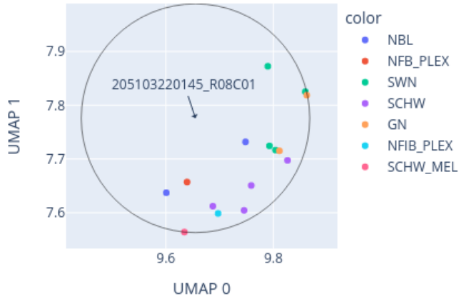
Close-up of UMAP for 205103220145_R08C01 reference: AllIDATv2_20210804_HPAP_Sarc.xlsx (19967 cases), 0 CpGs
