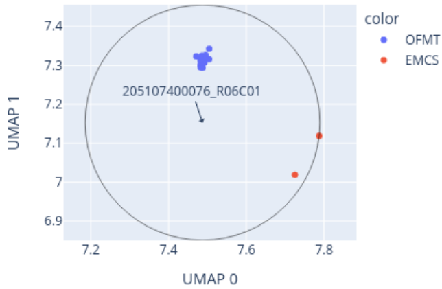
Close-up of UMAP for 205107400076_R06C01 reference: AllIDATv2_20210804_HPAP_Sarc.xlsx (19967 cases), 0 CpGs
