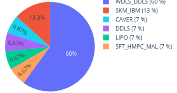
Neighbors in UMAP for 205121980079_R07C01 reference: AllIDATv2_20210804_HPAP_Sarc.xlsx (19967 cases), 0 CpGs
