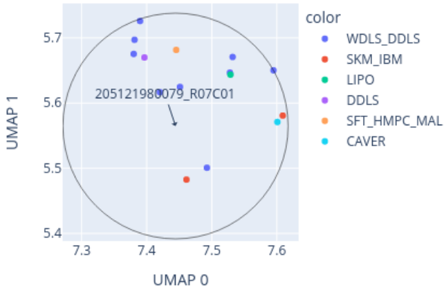
Close-up of UMAP for 205121980079_R07C01 reference: AllIDATv2_20210804_HPAP_Sarc.xlsx (19967 cases), 0 CpGs
