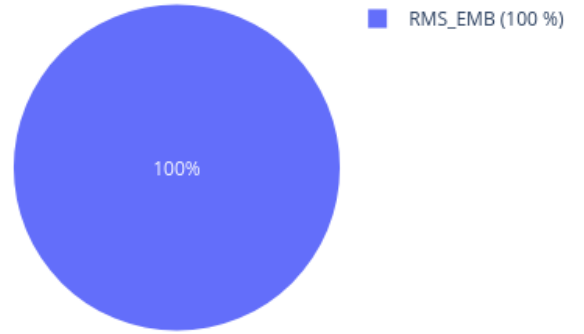
Neighbors in UMAP for 205138640081_R06C01 reference: AllIDATv2_20210804_HPAP_Sarc.xlsx (19967 cases), 0 CpGs
