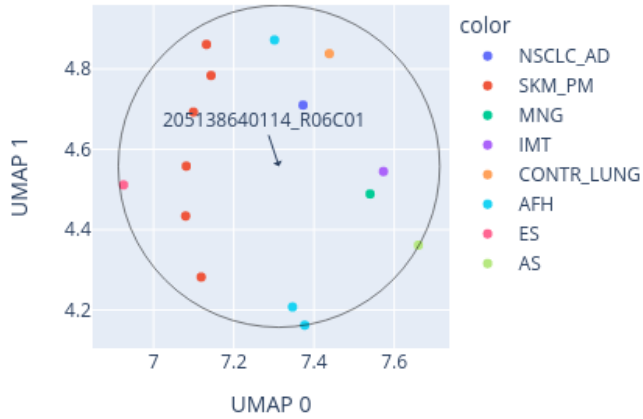
Close-up of UMAP for 205138640114_R06C01 reference: AllIDATv2_20210804_HPAP_Sarc.xlsx (19967 cases), 0 CpGs
