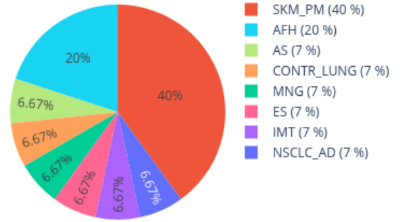
Neighbors in UMAP for 205138640114_R06C01 reference: AllIDATv2_20210804_HPAP_Sarc.xlsx (19967 cases), 0 CpGs
