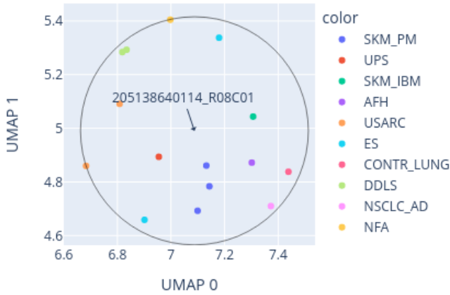
Close-up of UMAP for 205138640114_R08C01 reference: AllIDATv2_20210804_HPAP_Sarc.xlsx (19967 cases), 0 CpGs
