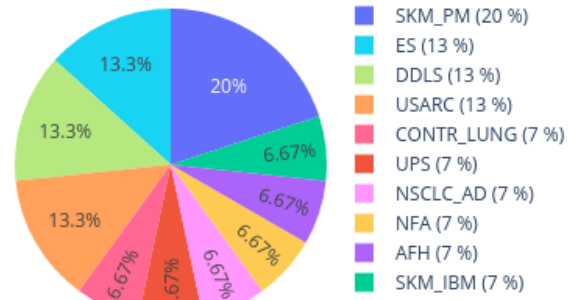
Neighbors in UMAP for 205138640114_R08C01 reference: AllIDATv2_20210804_HPAP_Sarc.xlsx (19967 cases), 0 CpGs
