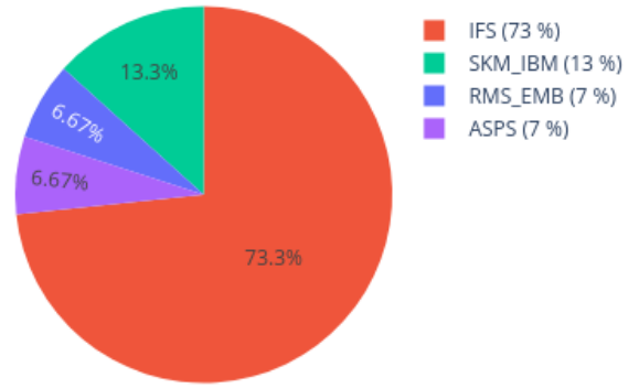
Neighbors in UMAP for 205379750058_R05C01 reference: AllIDATv2_20210804_HPAP_Sarc.xlsx (19967 cases), 0 CpGs
