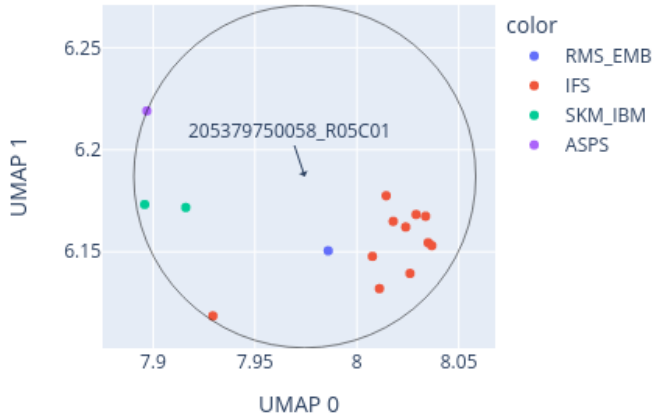
Close-up of UMAP for 205379750058_R05C01 reference: AllIDATv2_20210804_HPAP_Sarc.xlsx (19967 cases), 0 CpGs
