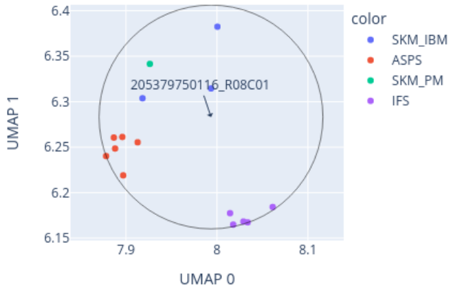
Close-up of UMAP for 205379750116_R08C01 reference: AllIDATv2_20210804_HPAP_Sarc.xlsx (19967 cases), 0 CpGs
