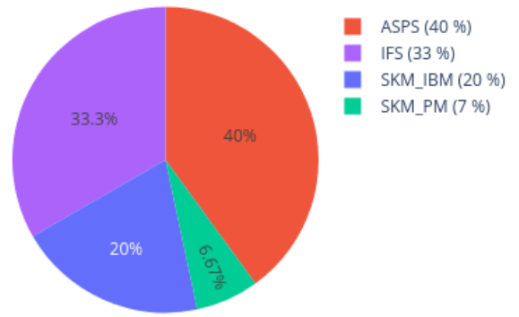
Neighbors in UMAP for 205379750116_R08C01 reference: AllIDATv2_20210804_HPAP_Sarc.xlsx (19967 cases), 0 CpGs
