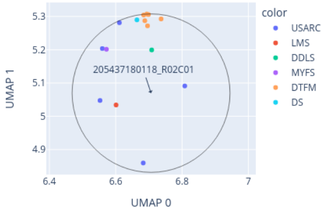
Close-up of UMAP for 205437180118_R02C01 reference: AllIDATv2_20210804_HPAP_Sarc.xlsx (19967 cases), 0 CpGs
