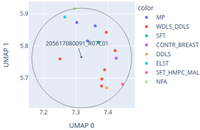
Close-up of UMAP for 205617080091_R07C01 reference: AllIDATv2_20210804_HPAP_Sarc.xlsx (19967 cases), 0 CpGs
