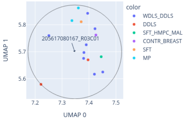
Close-up of UMAP for 205617080167_R03C01 reference: AllIDATv2_20210804_HPAP_Sarc.xlsx (19967 cases), 0 CpGs
