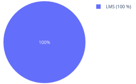
Neighbors in UMAP for 205624880105_R05C01 reference: AllIDATv2_20210804_HPAP_Sarc.xlsx (19967 cases), 0 CpGs
