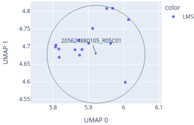
Close-up of UMAP for 205624880105_R05C01 reference: AllIDATv2_20210804_HPAP_Sarc.xlsx (19967 cases), 0 CpGs
