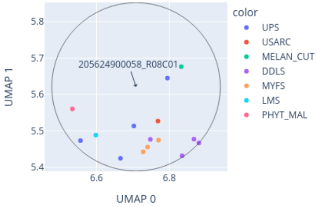
Close-up of UMAP for 205624900058_R08C01 reference: AllIDATv2_20210804_HPAP_Sarc.xlsx (19967 cases), 0 CpGs
