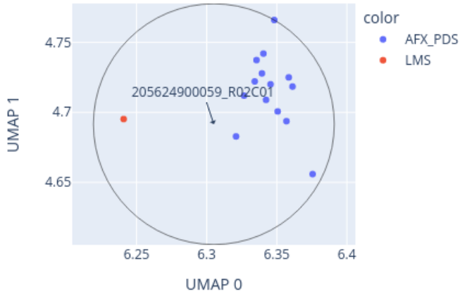
Close-up of UMAP for 205624900059_R02C01 reference: AllIDATv2_20210804_HPAP_Sarc.xlsx (19967 cases), 0 CpGs
