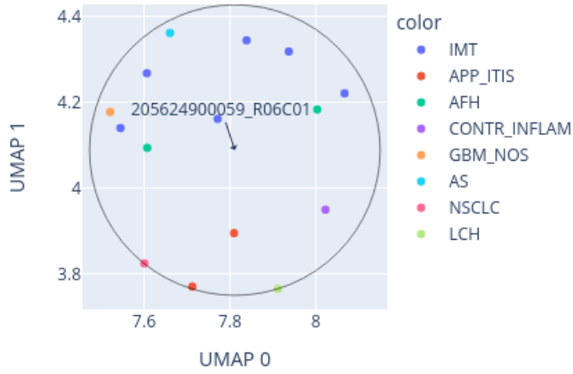
Close-up of UMAP for 205624900059_R06C01 reference: AllIDATv2_20210804_HPAP_Sarc.xlsx (19967 cases), 0 CpGs
