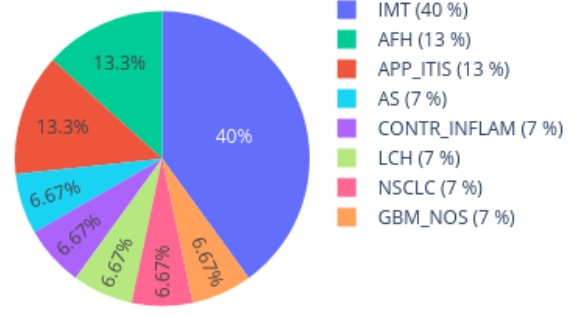
Neighbors in UMAP for 205624900059_R06C01 reference: AllIDATv2_20210804_HPAP_Sarc.xlsx (19967 cases), 0 CpGs
